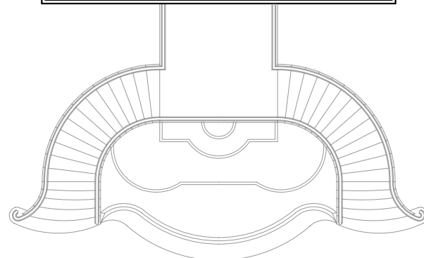
WALKER RESIDENCE, SECND FLOOR PLAN
