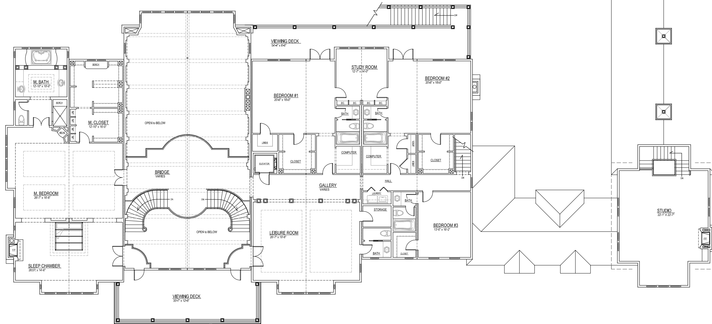
WALKER RESIDENCE, SECND FLOOR PLAN
