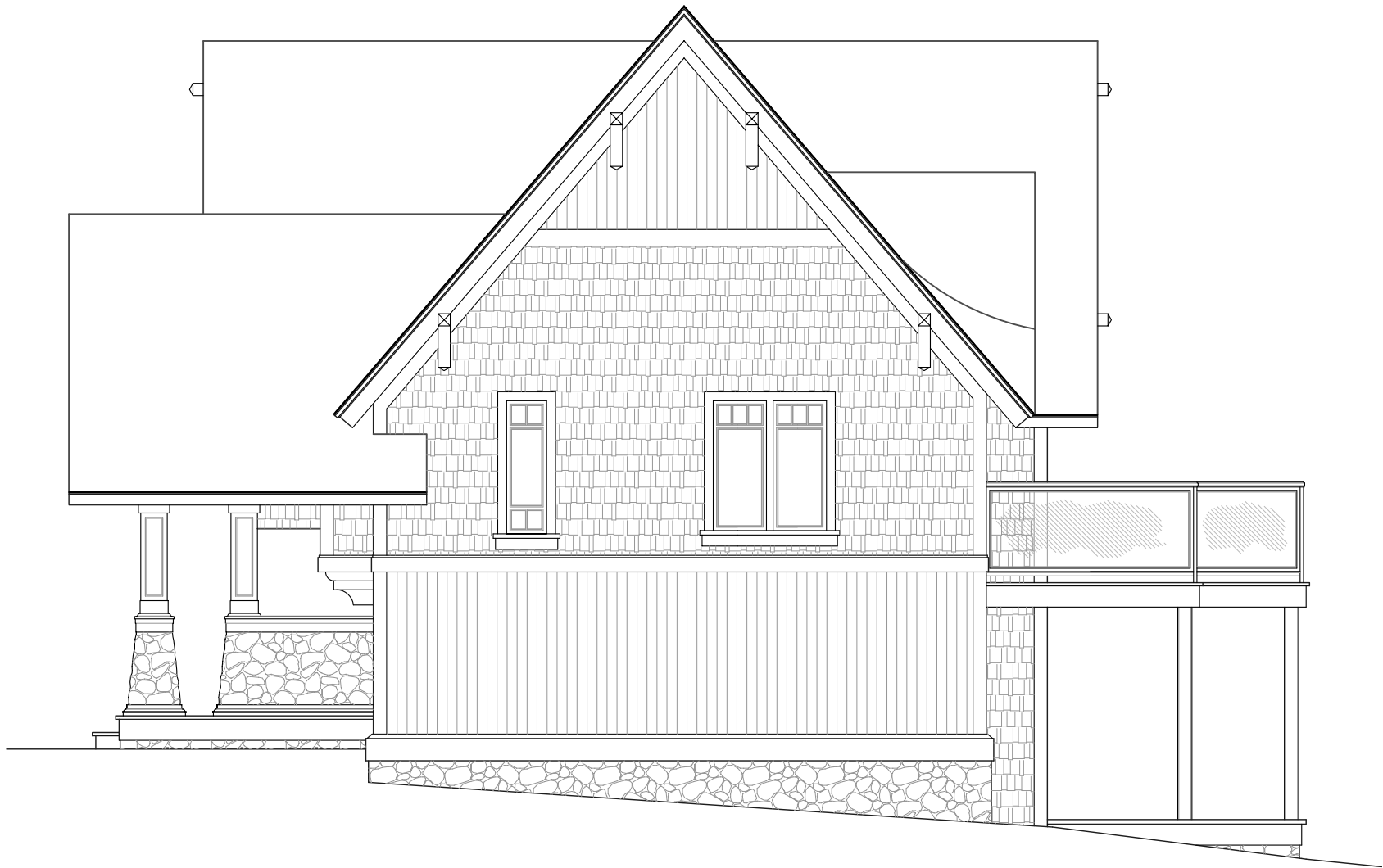
SAN JUAN 1, RIGHT ELEVATION, FACING
