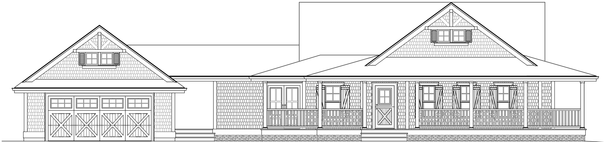
THE OAK (b), FRONT ELEVATION (with GARAGE)
