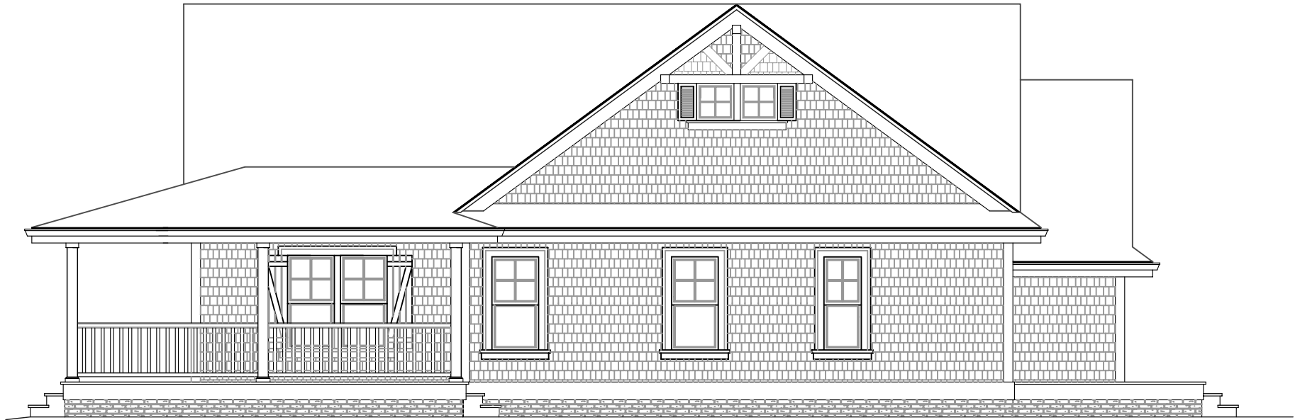
THE OAK (b), RIGHT ELEVATION, FACING (with GARAGE)
