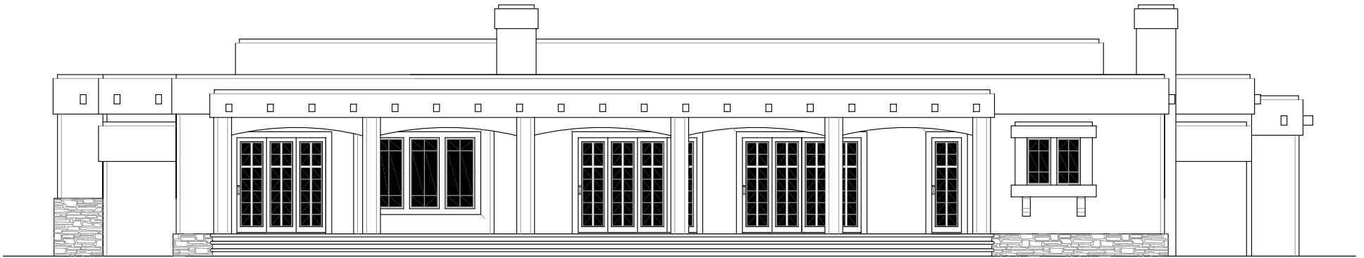
MESA VERDE, REAR ELEVATION
