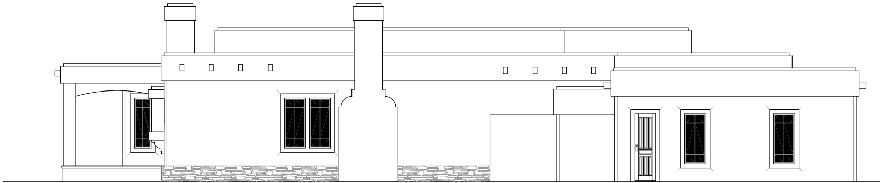
MESA VERDE, LEFT ELEVATION, FACING
