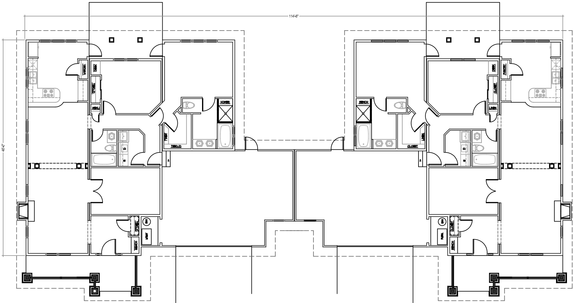
FOUNTAIN HILLS NO. 2, DUPLEX, FLOOR PLAN
