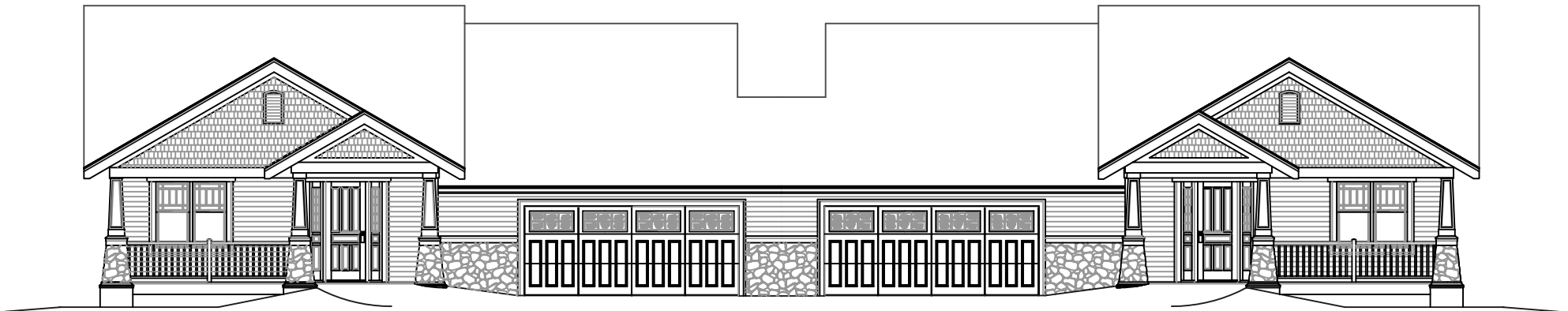
FOUNTAIN HILLS NO. 2, DUPLEX, FRONT ELEVATION
