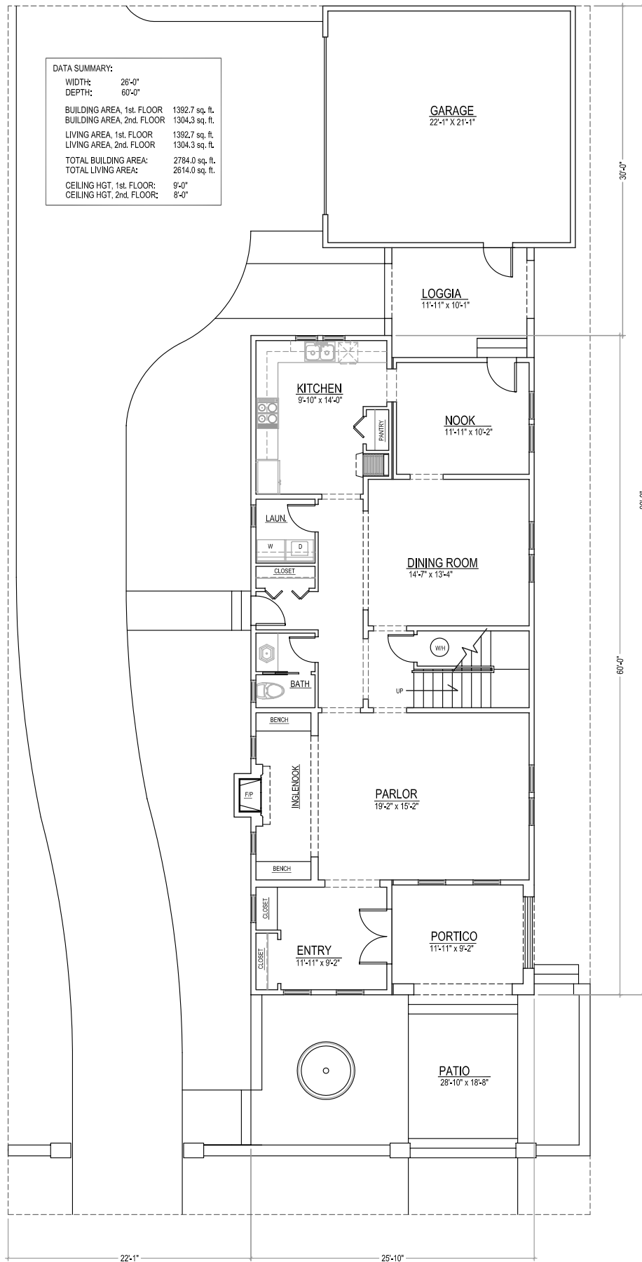
FIORENZA (b), FIRST FLOOR PLAN
